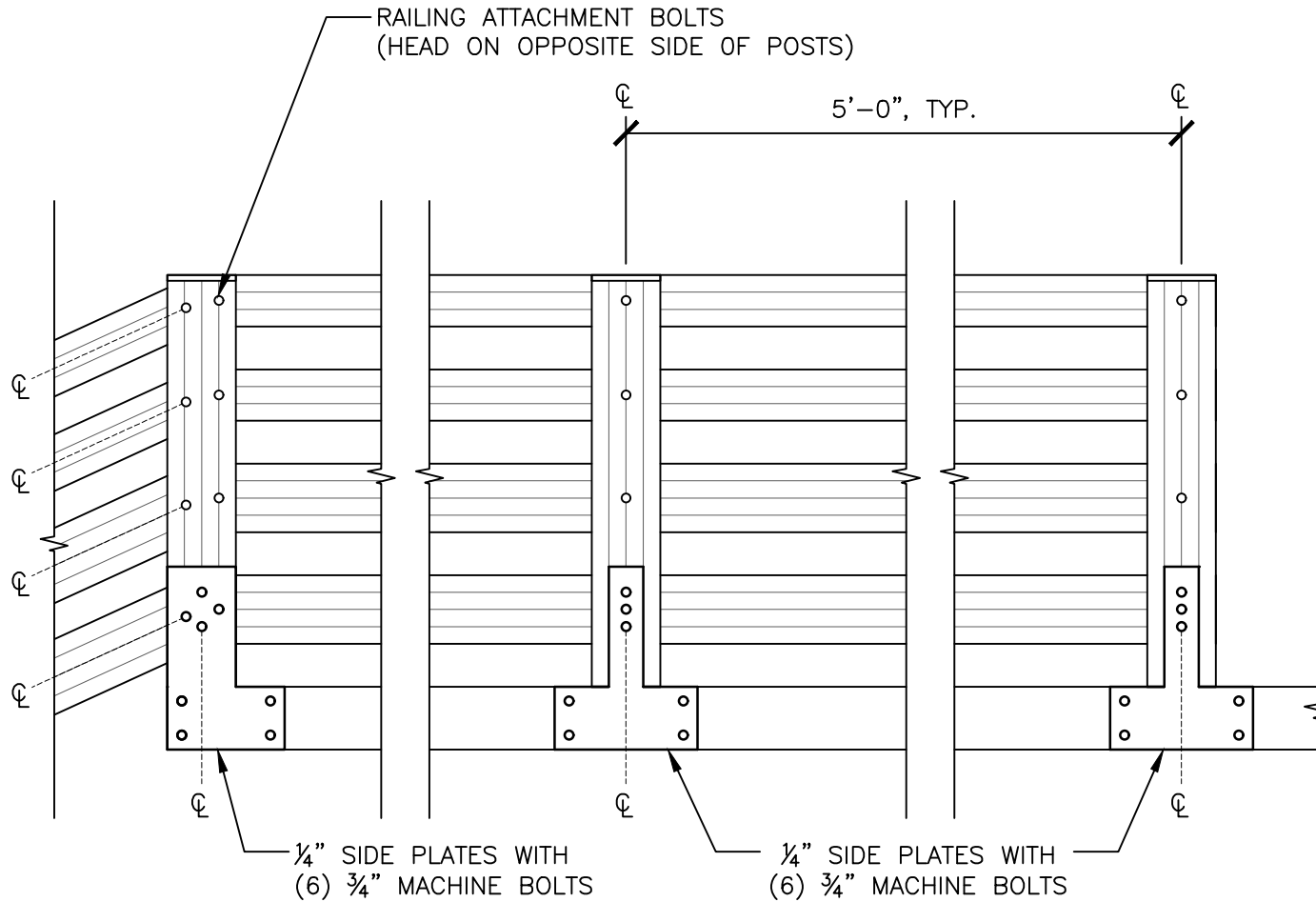
OUTSIDE ELEVATION AT LANDING/STAIR INTERFACE
