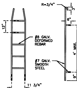
PREFABRICATED LADDER
