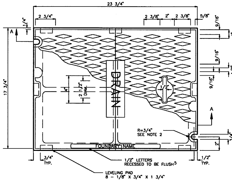
PLAN COVER
